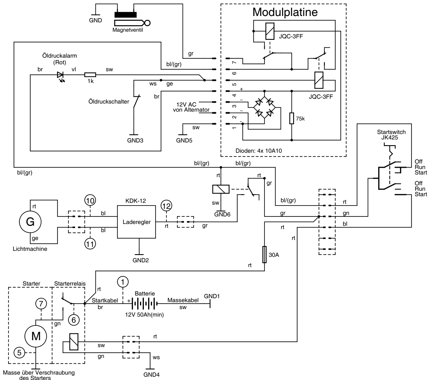
Rotek GD4W-3-012kW-EBDCZ Control Wire Schematic 04/2007
