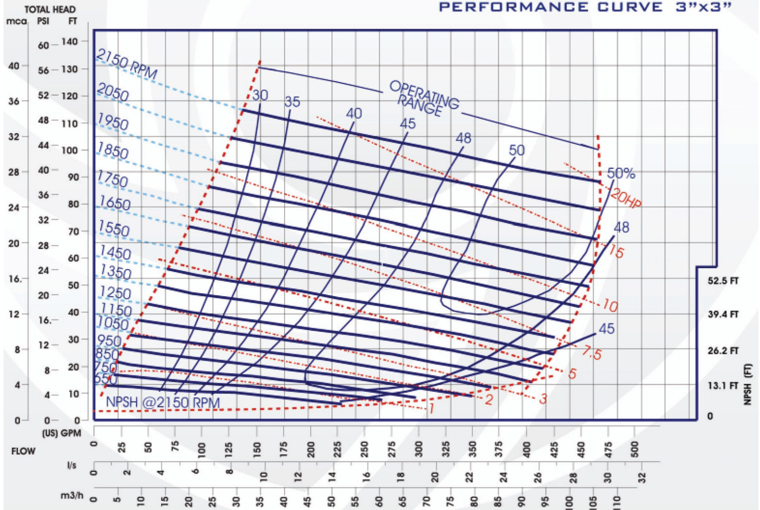
PERFORMANCE CURVE 3"x3"
