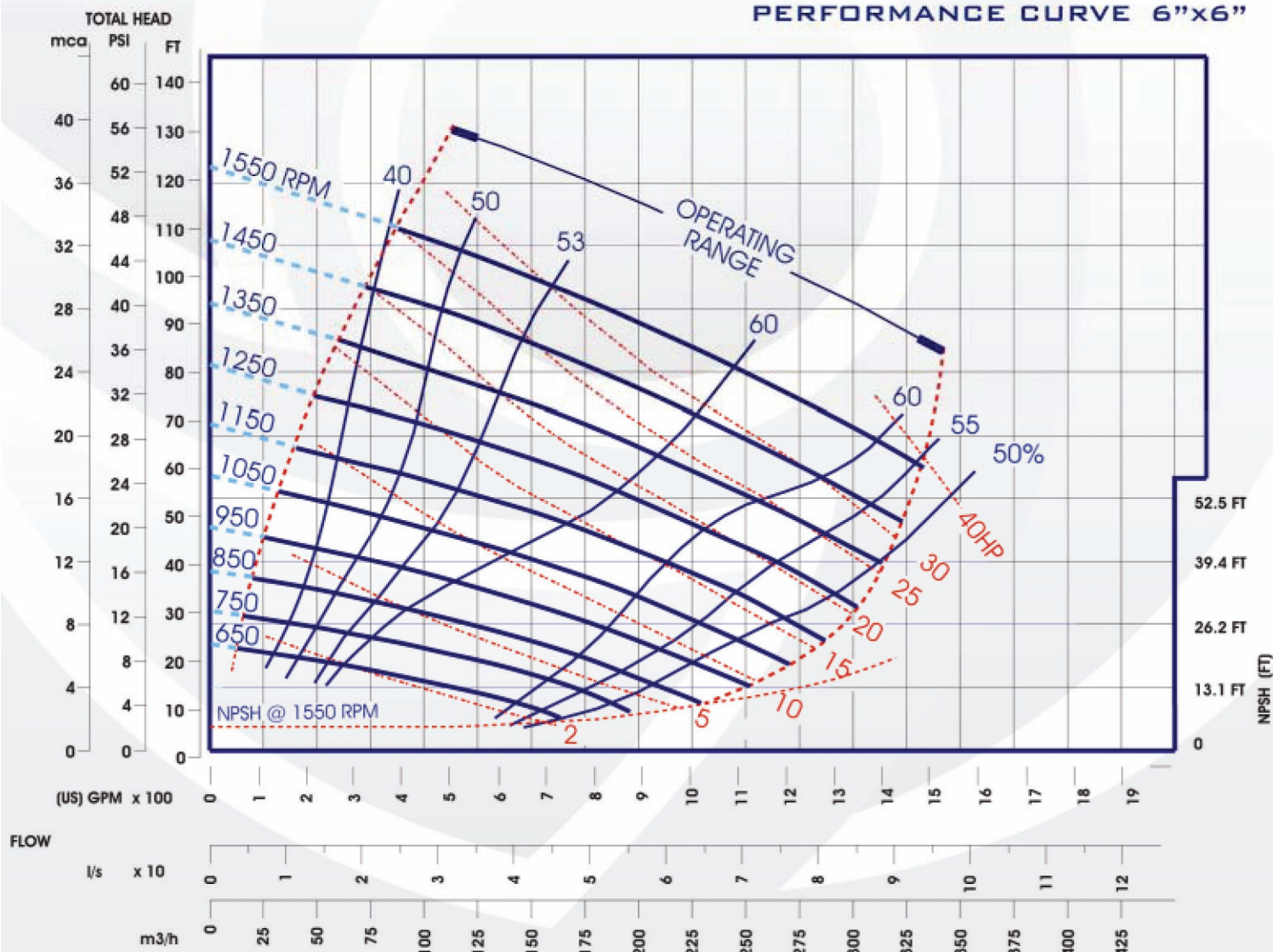
PERFORMANCE CURVE 6"x6"
